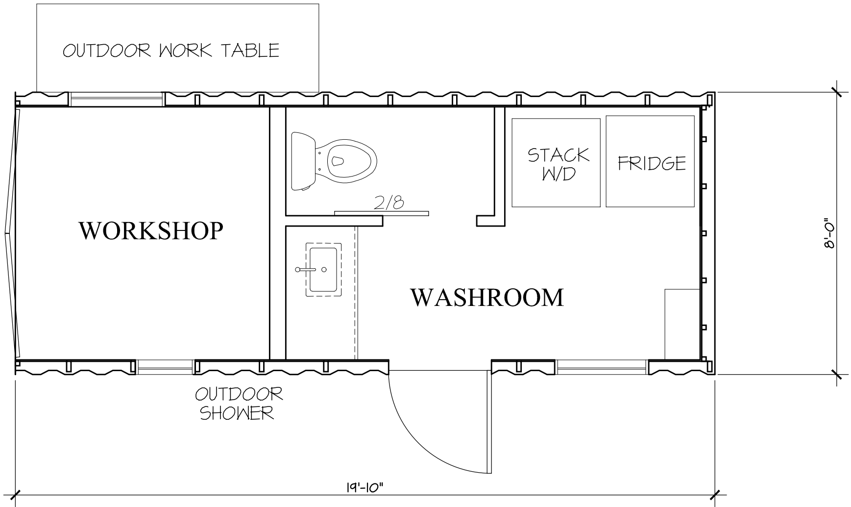
FLOOR PLAN - WASHROOM
