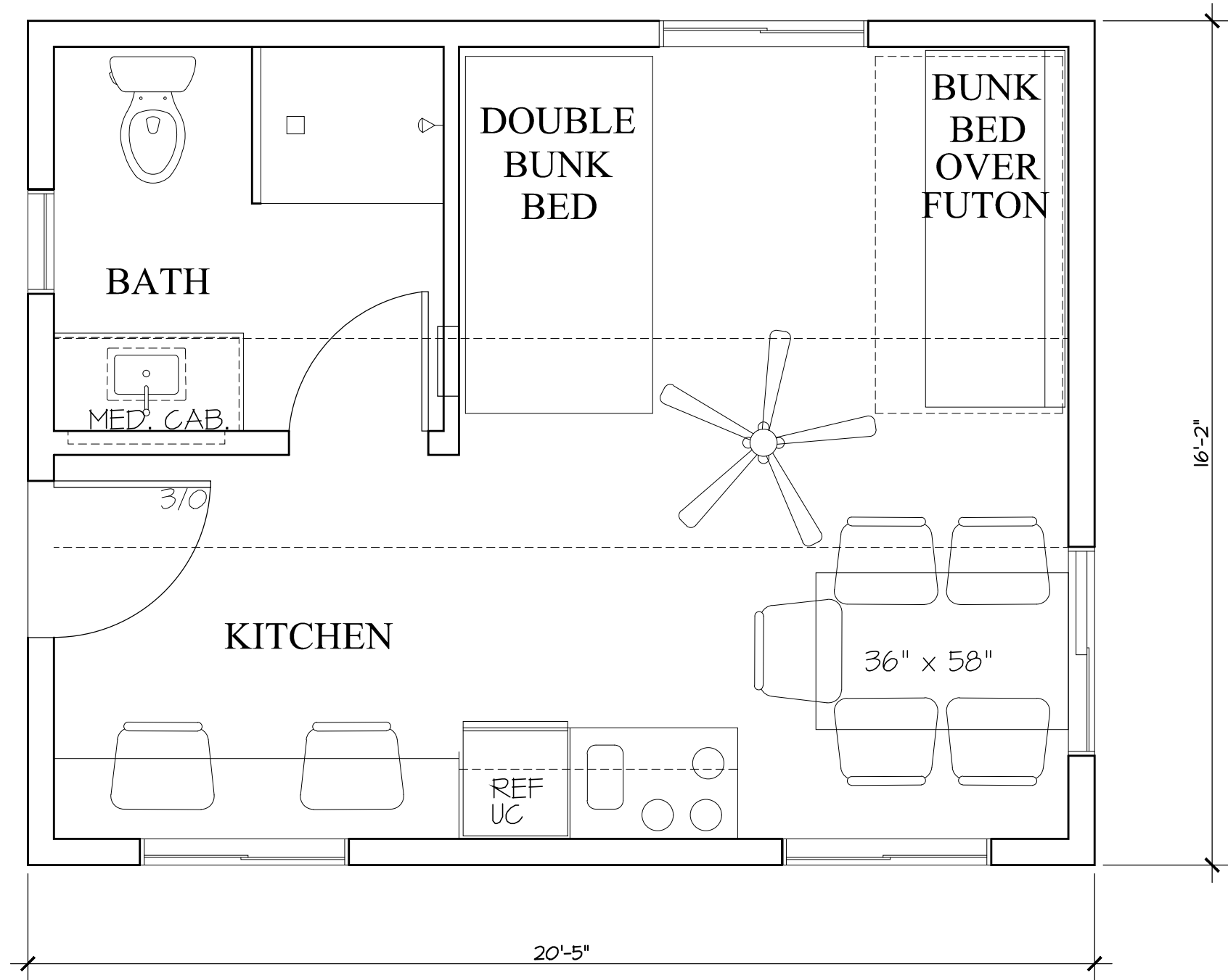
FLOOR PLAN CABIN
